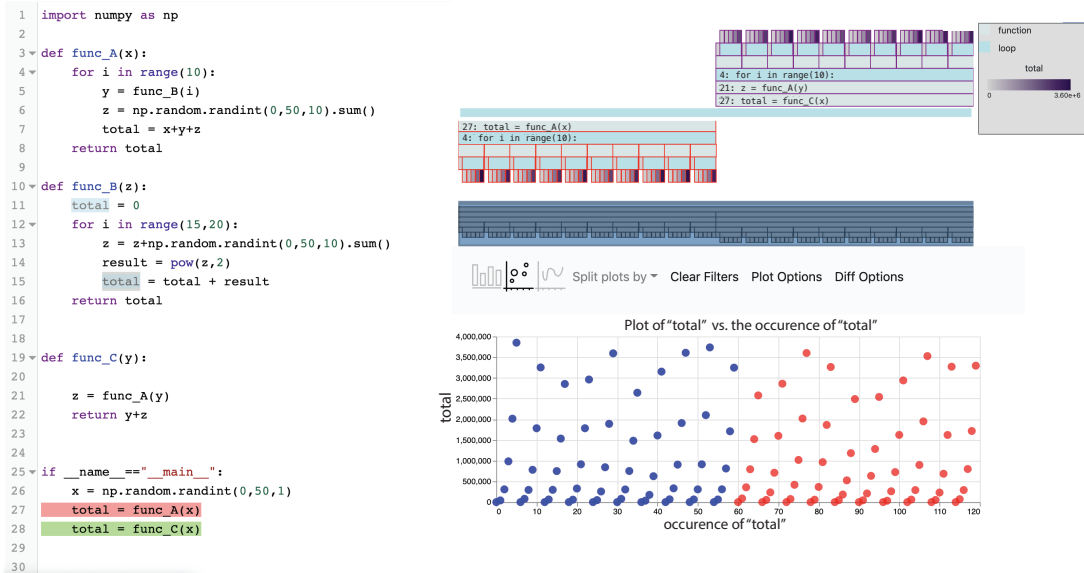
Figure 3.2: The execution diff of a program after we wrap the initial function call to func_A in a call to func_C . Doing this changes the depth of the call to func_A , causing this call and all subsequent children to be marked as additions.
