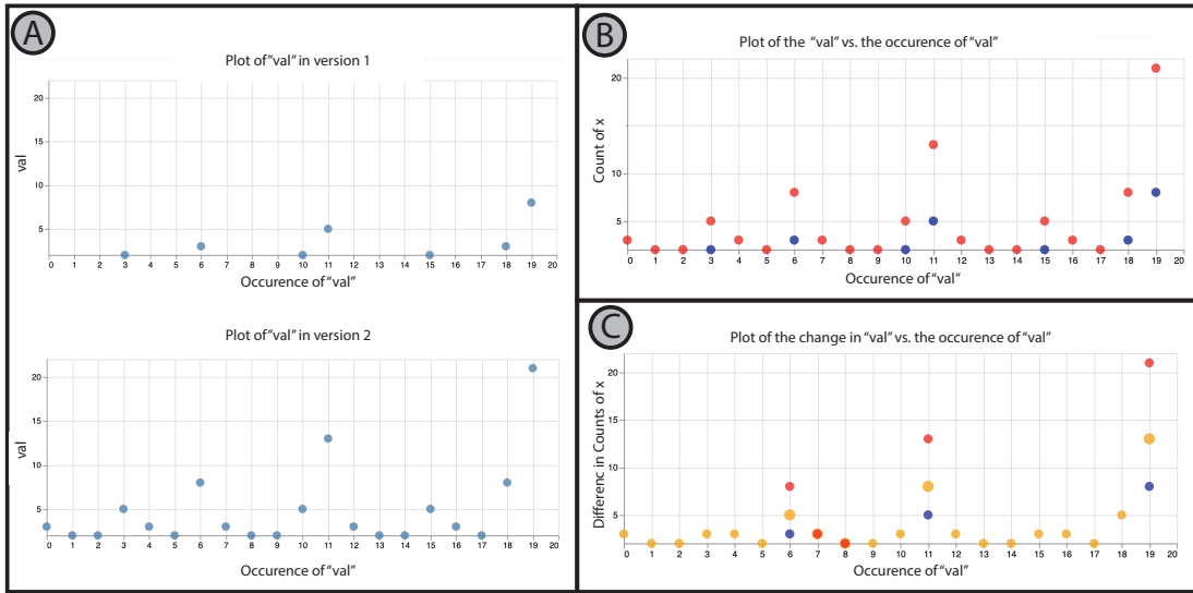
Figure 3.5: The comparative scatterplot views. The x-axis represents the occurrence (or instance) in the execution of the shown value. (A) shows the juxtaposition view. The top plot shows the scatterplot from the original trace and the bottom plot shows the scatterplot from the trace of the modified program. (B) shows the superposition view. We color points from the original version blue and points from the modified version red. Occurrences with only one point indicate an addition or deletion of an occurrence. (C) shows the explicit encoding of the difference between the occurrence in the modified execution and the original occurrence. Gold points represent the difference between the two occurrences. Selecting a point shows the actual values from both versions (in red and blue). When clicking a point only shows one point, this indicates that the point was added or deleted.
