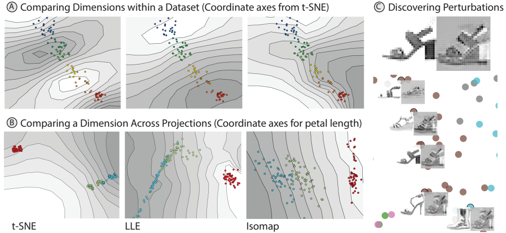
Figure 4.1: DimReader explains non-linear dimensionality reduction methods by illustrating the effects of user-designed perturbations of the input dataset. It provides an answer to the question “if the input data had been slightly different in a particular way, how would the plot have changed?”. In the case of traditional scatterplots, it recovers exactly the axis lines being displayed. In the case of non-linear methods, DimReader recovers generalized axes , which indicate how dimensions of interest behave. Examples of these axes are shown in (A) for the x, y, and z dimensions of the S Curve (an S shaped 3 dimensional manifold). These axes also allow for the comparison of different projection methods. This is exemplified in (B), where the petal length axis of the iris dataset is shown for three projections. Petal length is well behaved in t-SNE but not in the other projections. We also provide a technique for discovering good perturbations of the input (perturbations that change the projection the most). The top of (C) shows an example of a discovered perturbation. In context, shown at the bottom of (C), this perturbation shows us that t-SNE is sensitive to flat shoes v.s. heels. The perturbation wants to change the original image from a heel to a flat by filling in the arch.
