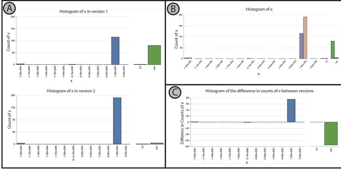
Figure 3.4: The comparative histogram views. (A) shows the juxtaposition view. The top plot shows the histogram from the original trace and the bottom plot shows the histogram from the trace of the modified program. (B) shows the superposition view. The left bars (colored purple for all quantitative values) represent the count from the original version and the right bar (colored orange) represent the count from the modified version of the program. (C) shows the explicit encoding of the difference of counts between the two traces. The count represents the count of the original version subtracted from the count of the modified version.
