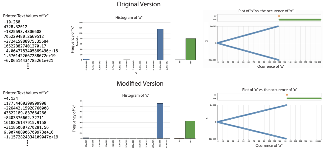
Figure 3.6: Current practices for comparing two program executions - the top row is the original execution and the bottom row is the execution after program modifications. . The first column shows the raw text values, as would be given by print statement debugging. The second and third columns present the visualizations from Anteater for both executions.
